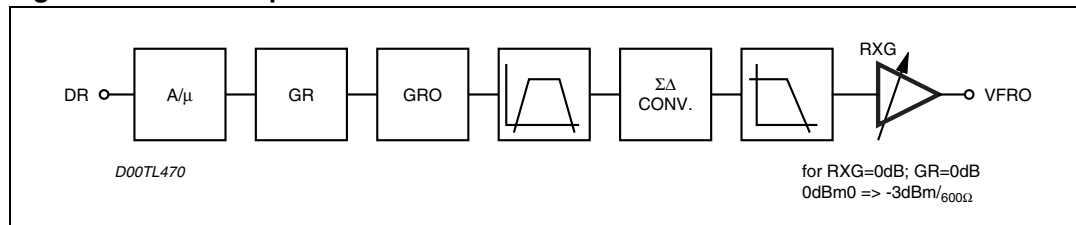
Figure 5. Receive path
