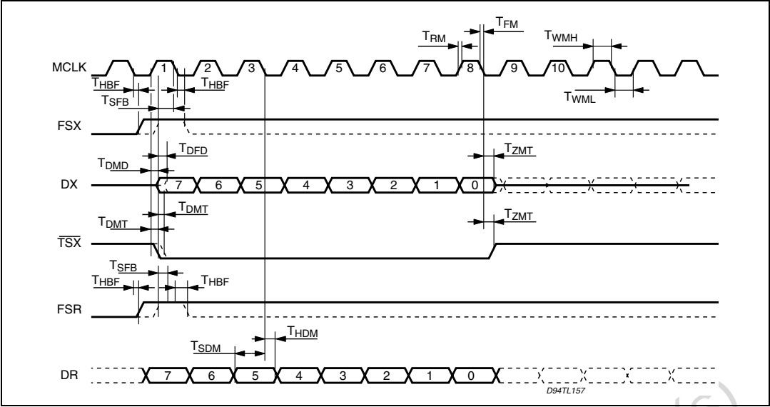
Figure 6. PCM interface timing
